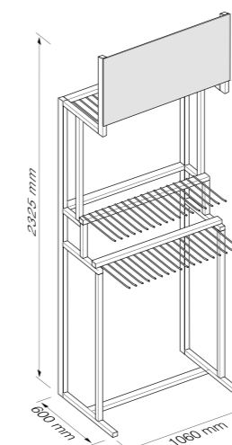
stojak Cirrus/Stratus
