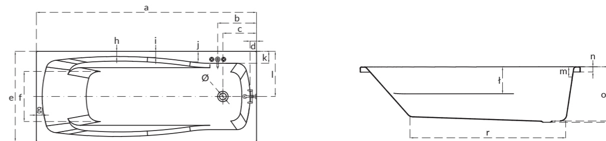
Wanna prostokątna LANA LANA rectangular bathtub
