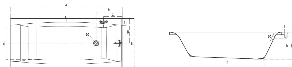
Wanna prostokątna VIRGO VIRGO rectangular bathtub
