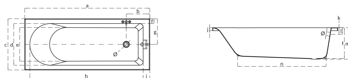
Wanna prostokątna FLAVIA FLAVIA rectangular bathtub
