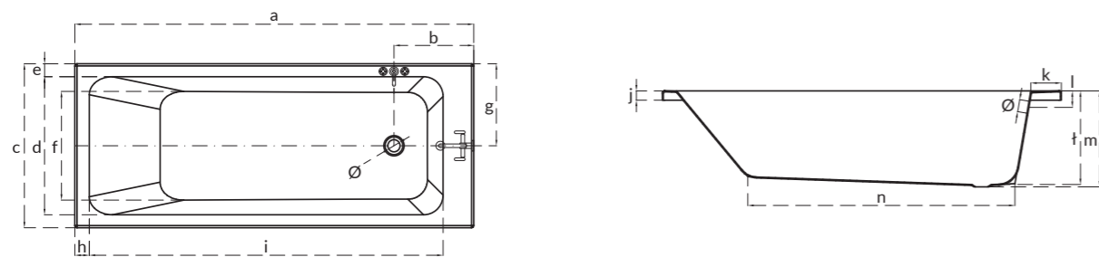
Wanna prostokątna BLISSA BLISSA rectangular bathtub
