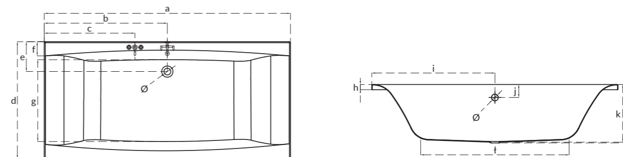
Wanna prostokątna VIRGO VIRGO rectangular bathtub
