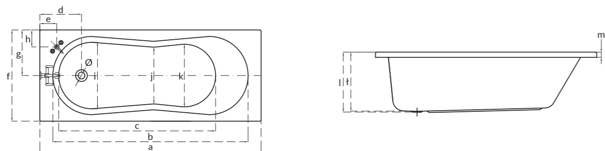
Wanna prostokątna NIKE NIKE rectangular bathtub
