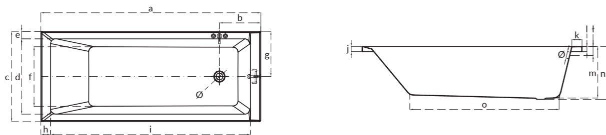
Wanna prostokątna BALINEA BALINEA rectangular bathtub
