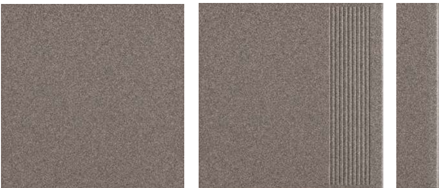
VIRGINIA salt-pepper matt size: 30x30 cm thickness: 0,72 cm VIRGINIA salt-pepper stair tread matt size: 30x30 cm thickness: 0,72 cm VIRGINIA salt-pepper skirting board matt size: 7,2x30 cm thickness: 0,72 cm
