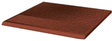
CLOUD ROSA DURO stair tread matt structure size: 30x30 cm thickness: 0,85 cm
