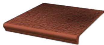
CLOUD ROSA DURO straight stair tread with bullnose matt structure size: 30x33 cm thickness: 1,1 cm
