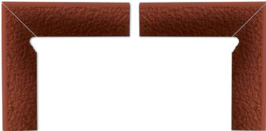
CLOUD ROSA DURO SKIRTING BOARD LEFT size: 8,1x30 cm thickness: 0,85 cm
