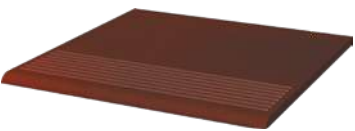
CLOUD BROWN stair tread matt size: 30x30 cm thickness: 0,85 cm
