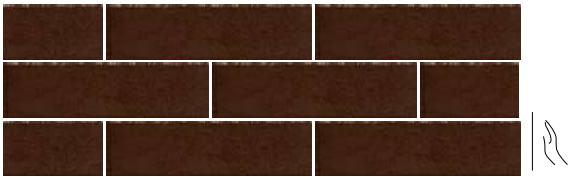
SUNDOWN MARRONE elevation glossy structure size: 6,6x24,5 cm thickness: 0,7 cm
